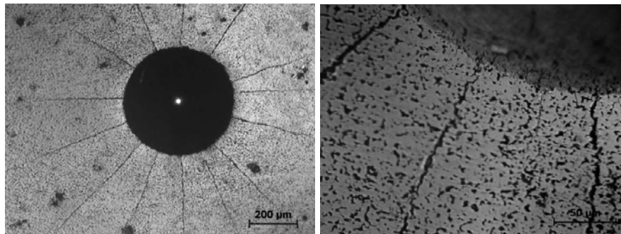
Fig. 8. Rockwell indentation image made on C45 steel after borocopperizing (2% Cu)
