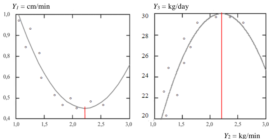
Fig. 2. The graphs of the electrical conductivity of milk Y_1 (a) and milking Y_3 (b) at the milk flow rate Y_2 [ Y_1 ] = cm/min; [ Y_2 ] = kg/min; [ Y_3 ] = kg/day
