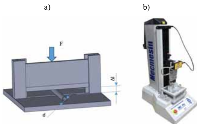
Fig. 1. Scheme of the tests (a) and testing machine Mecmesin (b)
