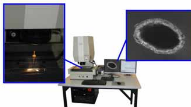
Fig. 3. Measurement of cross-sectional area on the optical measuring machine Werth
