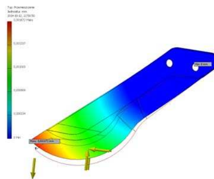
Fig. 11. Determined displacement of the coulter based on computer simulation [9]
